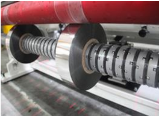
Rewinding Slipping Shaft
