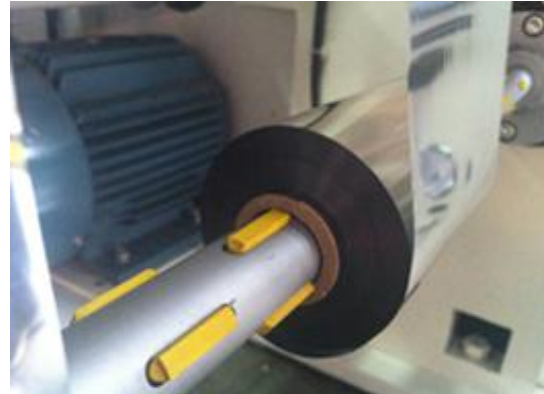
Rewinding Normal Air Shaft 1"
